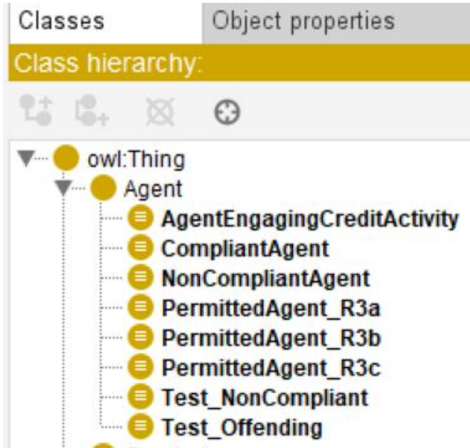
Figure 5: Main classes related to Agent
