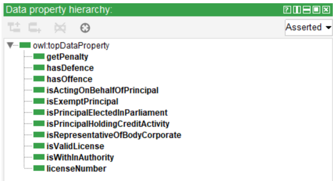
Figure 3 Data Properties Hierarchy
